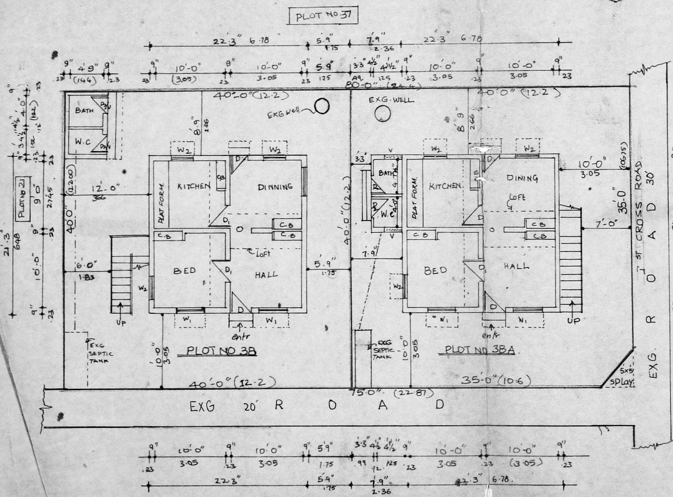
SUB-DIVISION PLAN
